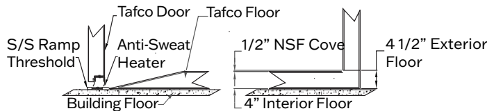
Floor Type 1 with Internal Ramp
